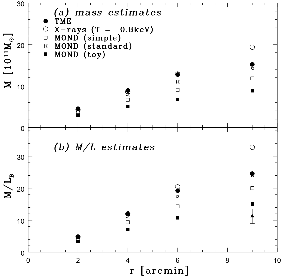
Fig. 1. Total Newtonian and MOND masses (upper panel) and Newtonian and MOND mass-to-light ratio, (lower panel). In the Newtonian approach we used "tracer mass estimates" and X-ray halo with temperature T = 0.80 keV, according to the observational data of Randall et al. (2006). In the MOND approach we tested three different models: "simple", "standard", and Bekenstein's "toy" model (see text for details). Additional point in the lower panel at 9 arcmin (given by the filled triangle) corresponds to the MOND estimate of the total mass-to-light ratio based on the "toy" model and the TME methodology. The distance d = 15.96 Mpc is used throughout.
