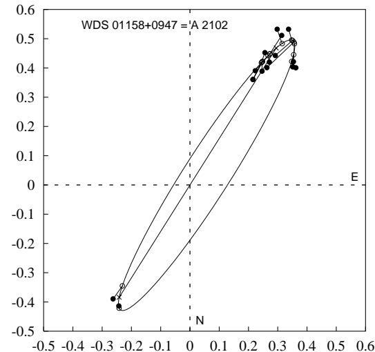
Fig. 1. Orbits of 12 visual binary stars. Coordinates are given in arcseconds.
