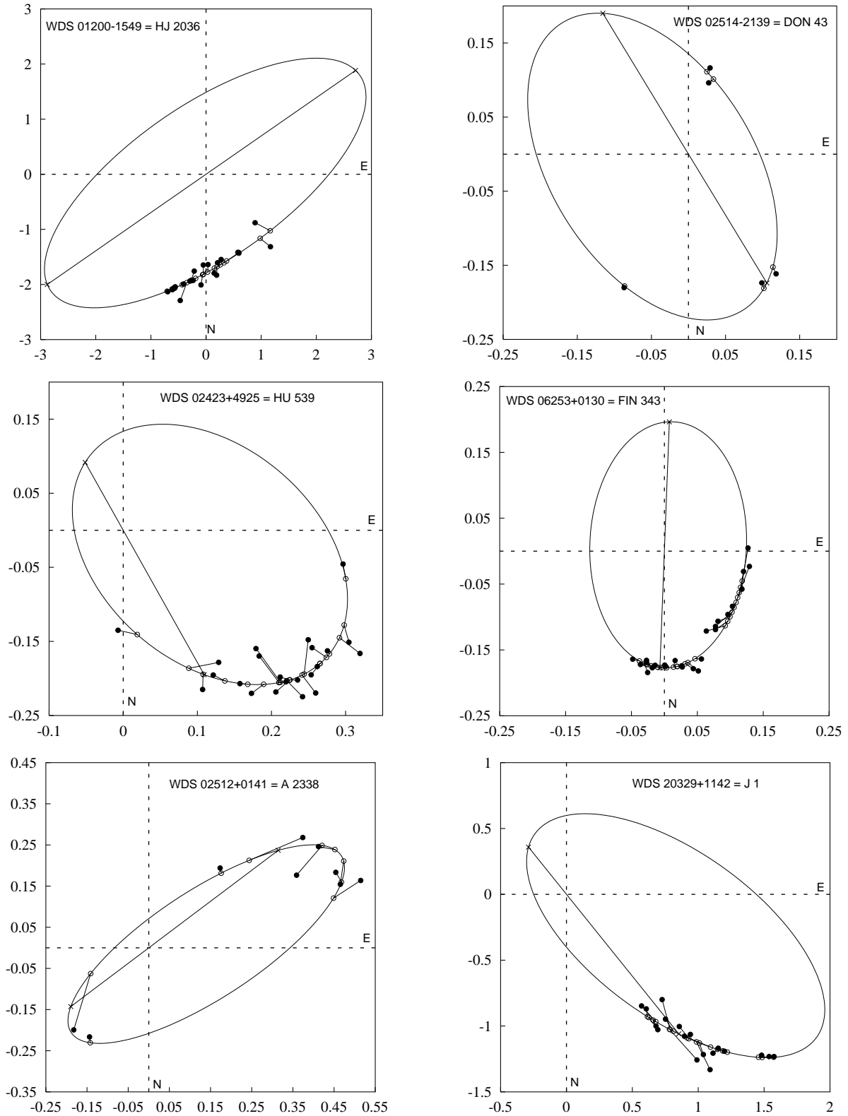
Fig. 1. Orbits of 12 visual binary stars (continued). Coordinates are given in arcseconds.
