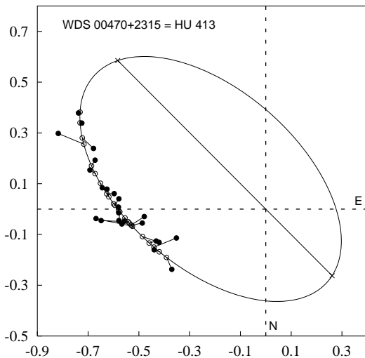
Fig. 1. Orbits of 12 visual binary stars. Coordinates are given in arcseconds.
